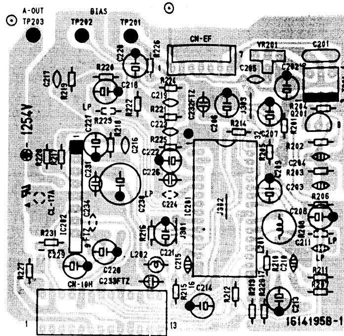
11-2-1 AUDIO P.C.BOARD TOP VIEW
