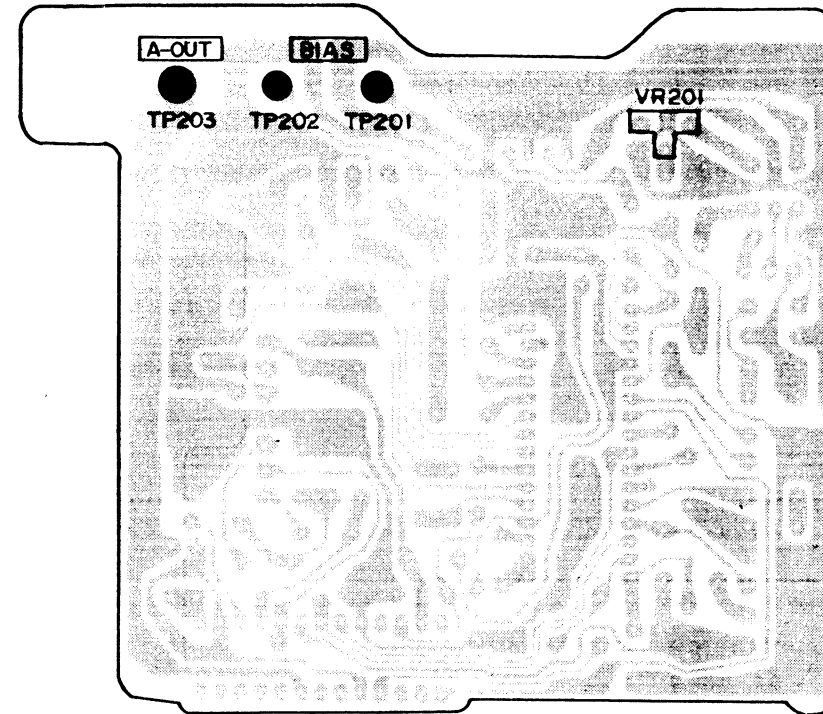
9-4 AUDIO P.C.BOARD VCR6000
