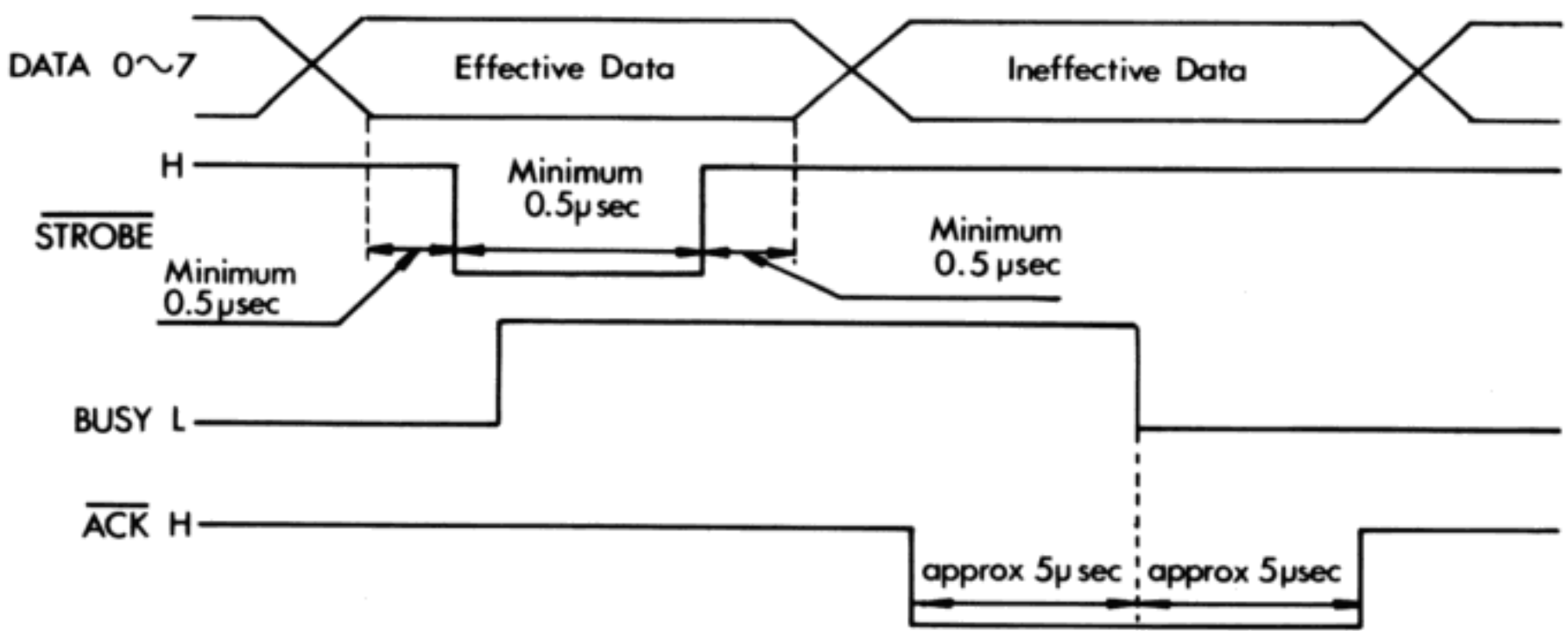
DATA input waveform
