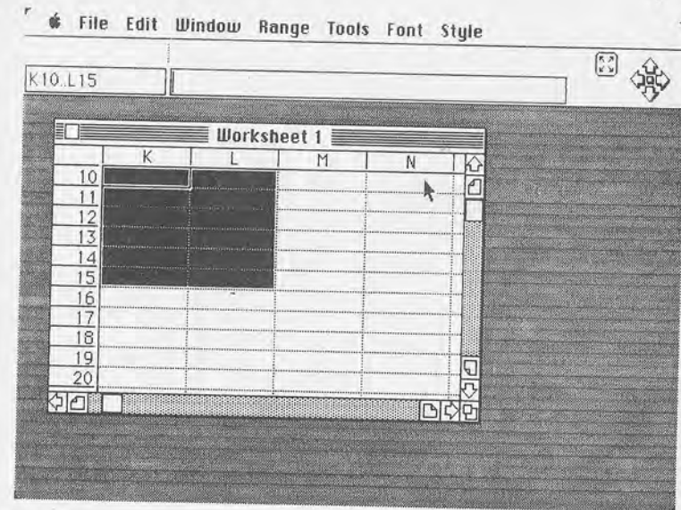
Figura 11.—Rango K10.L15
