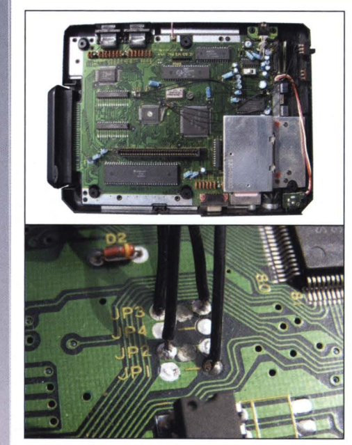
Two pathway cuts, four wires and two single-pole, double-throw switches. At ten minutes' work, this UK MD conversion opens up a plethora of Japanese software and is well worth the effort
