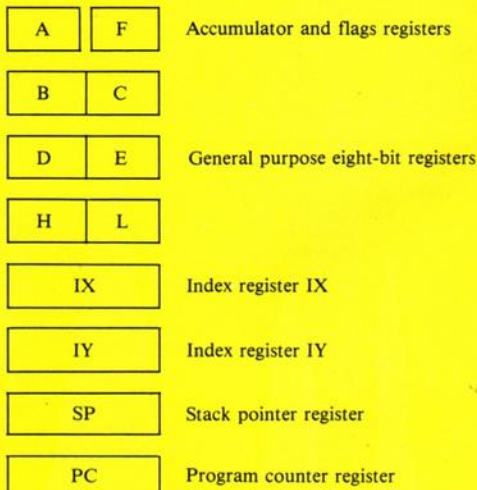
Figure 1. The Z80 registers
