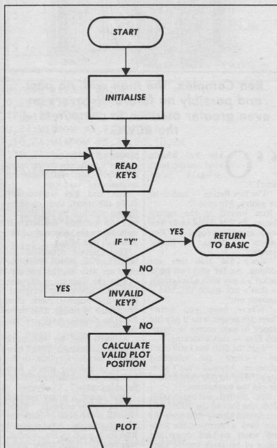
Fig 1 Flowsheet of "sketch" routine; see Part 6 Listing 1
