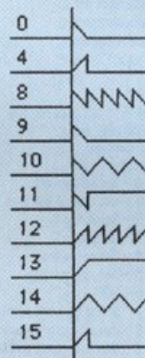
Fig 2 - Envelopes selected from sound chip register 13.
