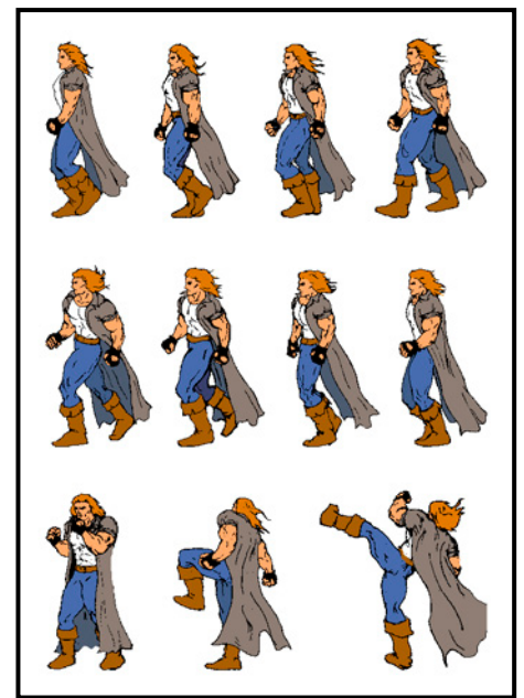
SPRITES - VAMPHIRE
