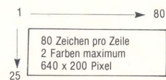
Text-Screen Mode 2
