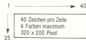
Text-Screen Mode 1
