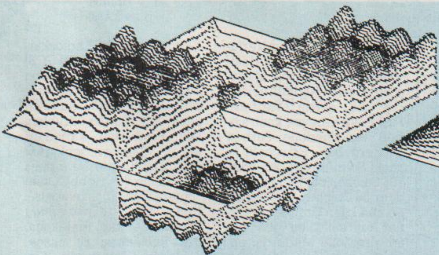
Beispiel 6: v_x = 0 , v_y = 0 , v_z = 35 , rg = 2 , sz = 25 Fkt. = 4/PI \star (\sin(PI \star x/75) - \sin(PI \star 6/150)/9 + \sin(PI \star 10/150)/25 - \sin(PI \star 14/150)/49) \star 4/PI \star (\sin(2 \star PI \star y/150) - \sin(PI \star 6/150)/9 + \sin(PI \star 10/150)/25 - \sin(PI \star 14/150)/49)
