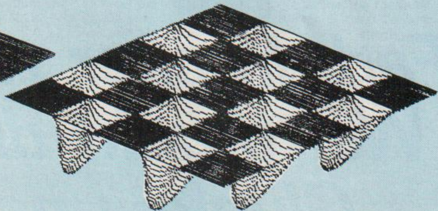
Beispiel 5: Funktion = \sin(0.1047 \star X) \star \sin(0.1047 \star y) v_x = 0 , v_y = 0 , v_z = 38 , ZM = 0 , sz = 40 , rg = 1
