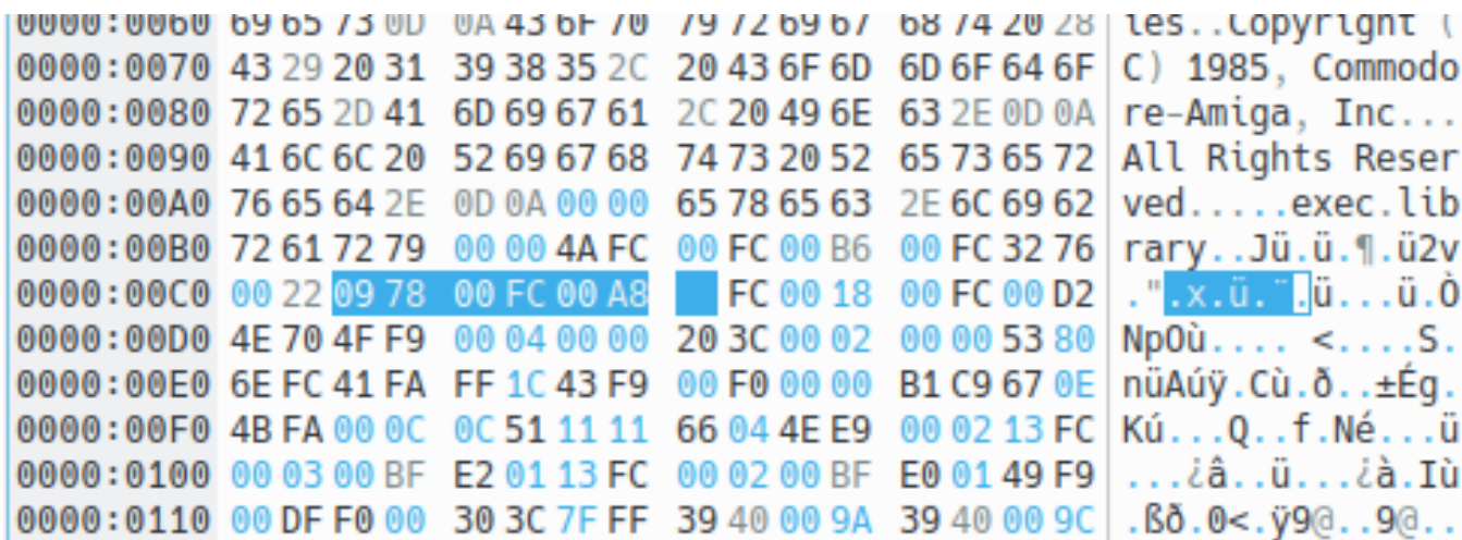
Figura 2 – Search Pattern string.
