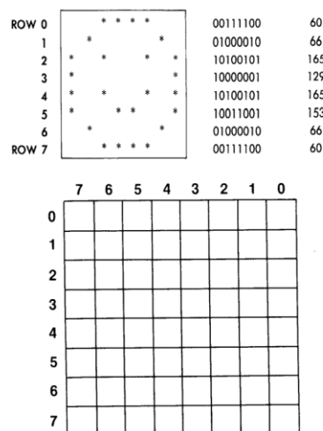
Figure 3-1. Programmable Character Worksheet.
